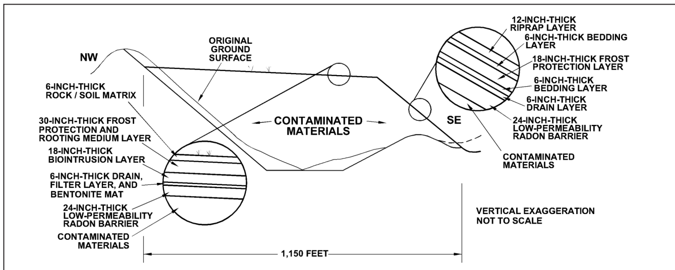
Northwest-Southeast Cross Section of the Durango Disposal Cell
